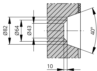
Bore in mould (if required) | Y
