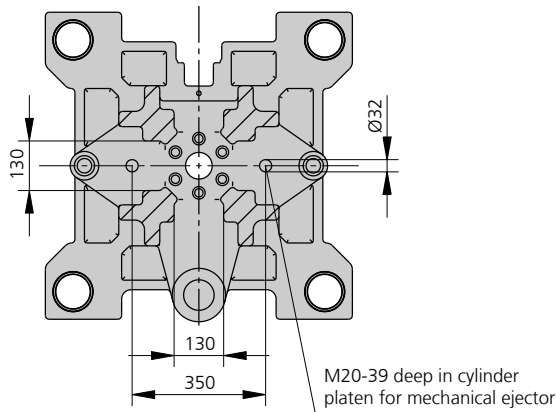
Ejector plate | D
