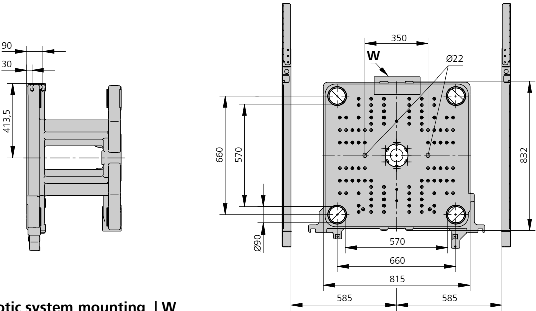
Robotic system mounting | W
