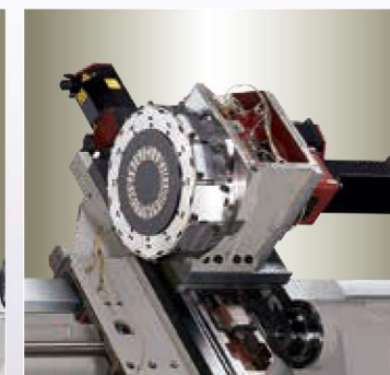
C axis BMT 75 turret (CM)
