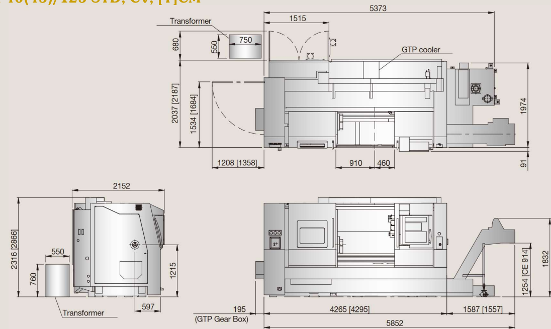
Vturn-40(45)/125 STD, CV, [Y]CM
