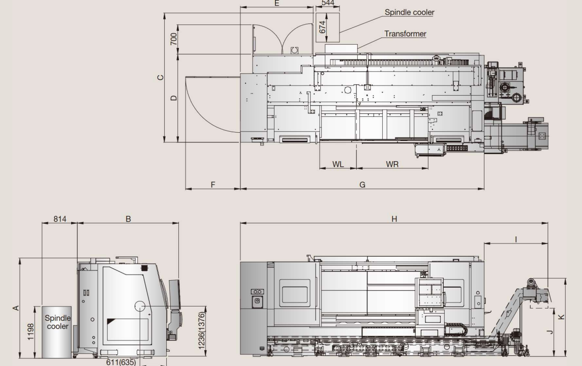
Vturn-40/220, 325, 425 [Y]CM with built-in spindle
