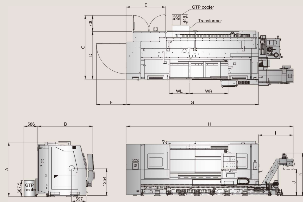
Vturn-40(45)/220, 325, 425 STD, CV, [Y]CM
