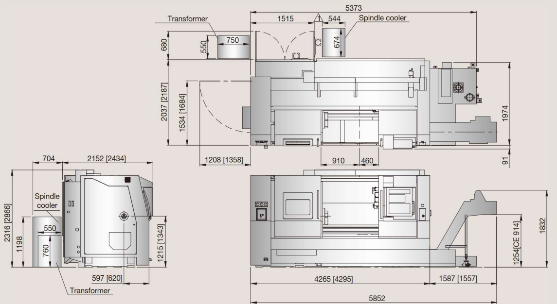
Vturn-40/125 with built-in spindle (CV, [Y]CM)
