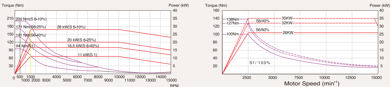
Siemens motor 1PH8131 (optional) Vcenter-AX380/AX630
